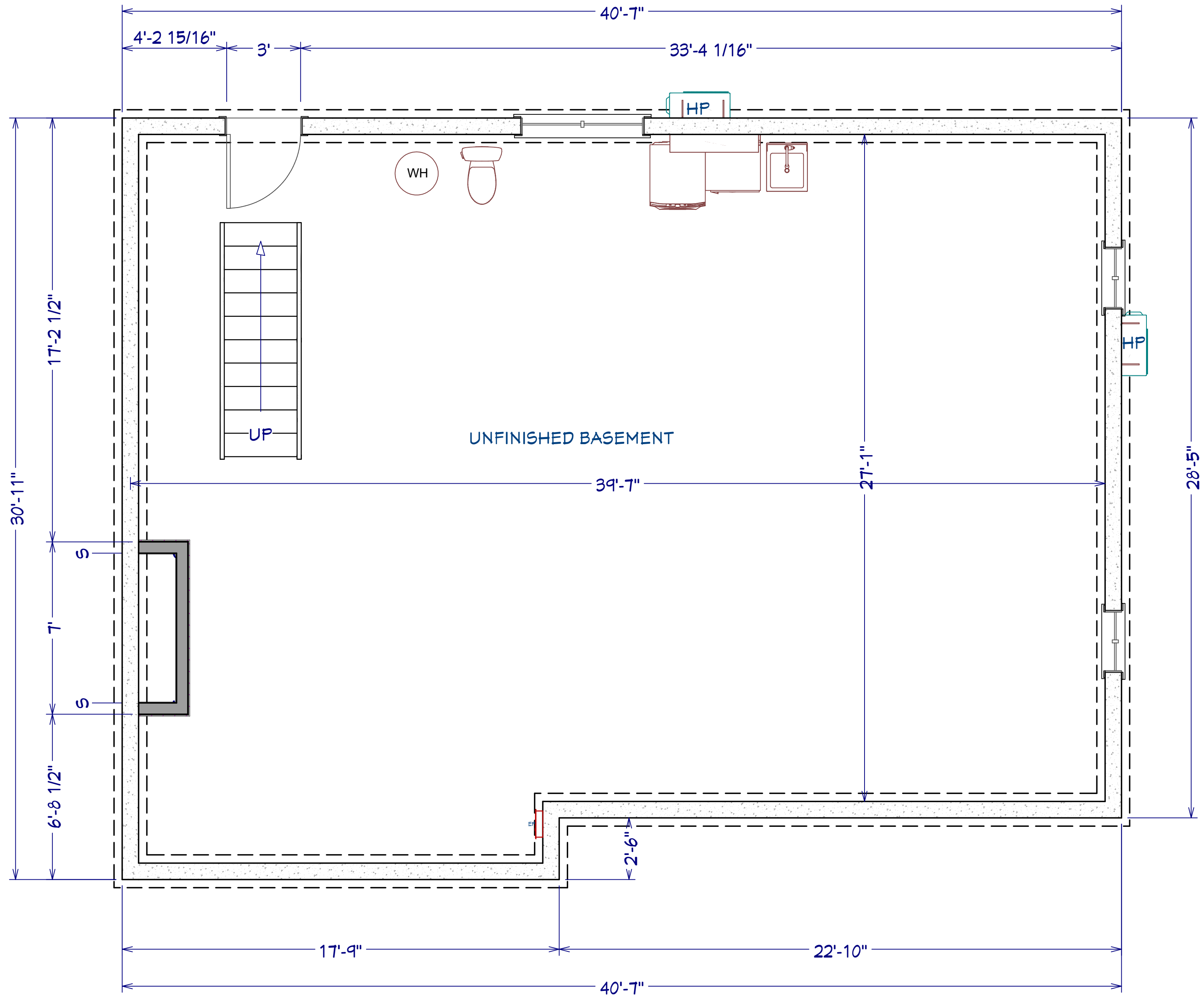
UNFINISHED BASEMENT LIVING AREA 1184 SQ FT
